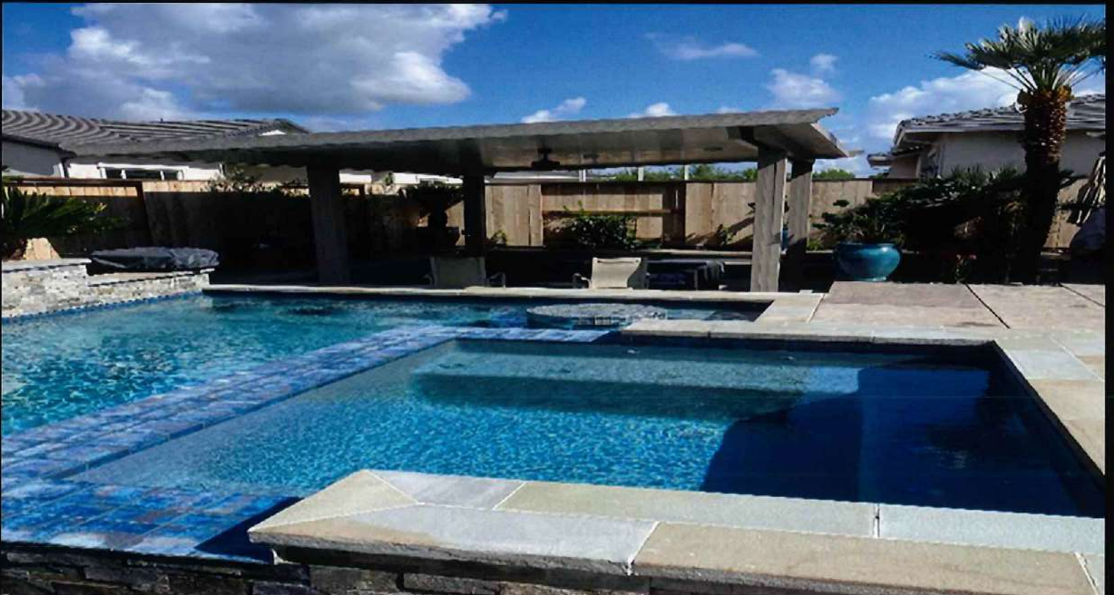
Driftwood IRP with double 3x8 beams, 2x6 wrap, 8x9 post, and 8x8 steel baseplates.
